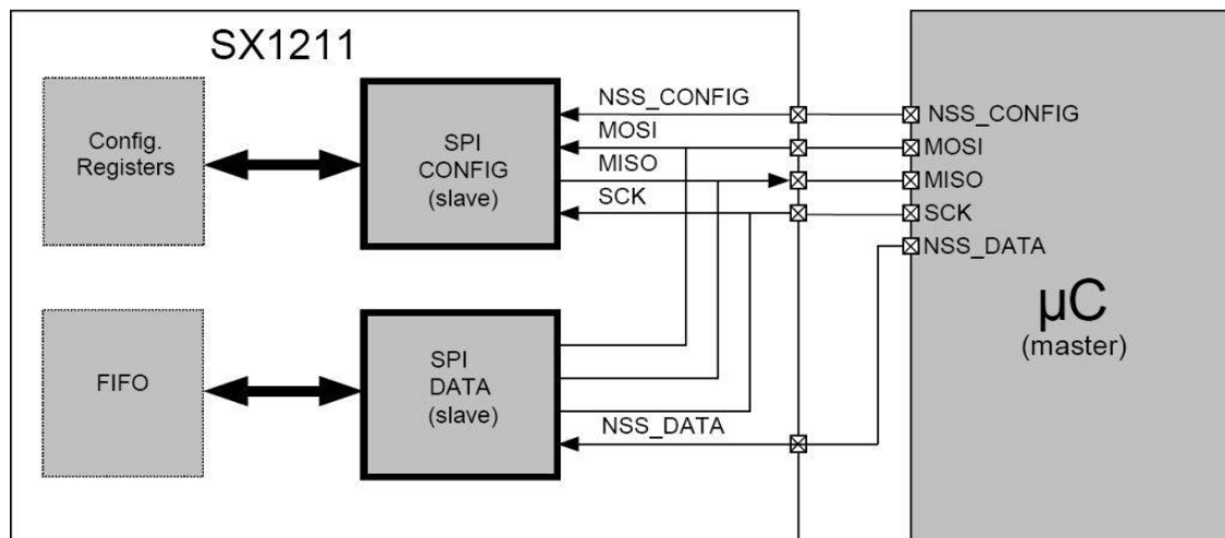
SPI Interface Overview and \mu C Connections
